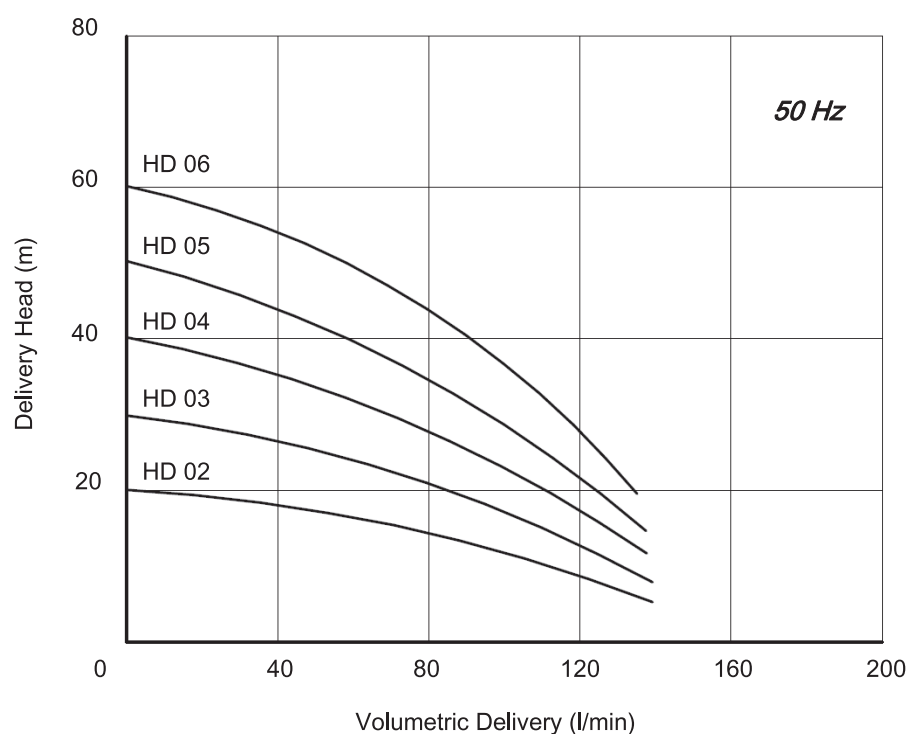
Performance Curve
