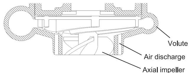
JB H 200 - Axial front impeller with air release
