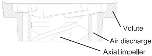
IPH - Axial front impeller with air release
